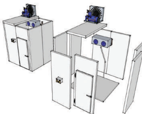
COLD ROOMS
